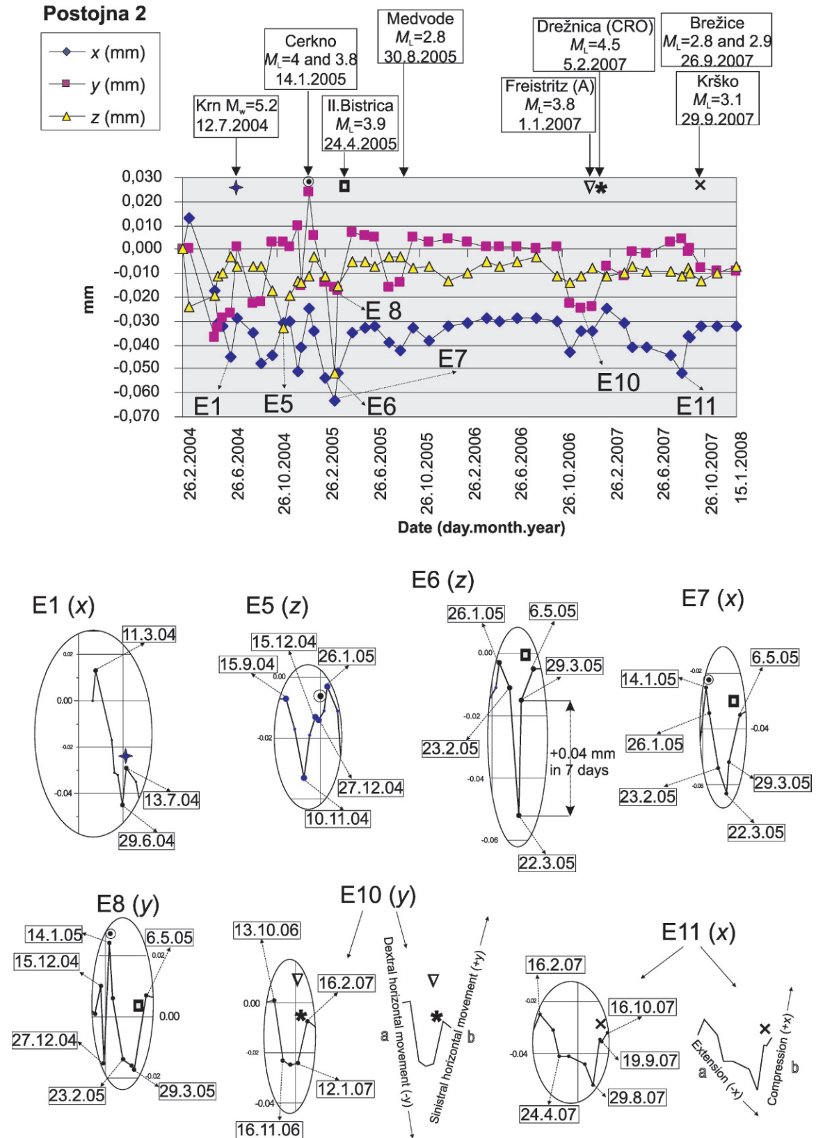
Figure 6. Displacements recorded by TM 71 at Postojna 2 monitoring site.
