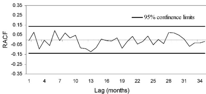
Figure 6. RACF for the selected ARIMA (1,0,1)(0,1,1) 12 monthly model for the Sangsourakh Hydrometric Station.
