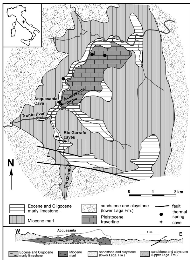
Figure 1. Geologic map of the study area. Geologic section after Scisciani and Montefalcone (2005), simplified.
