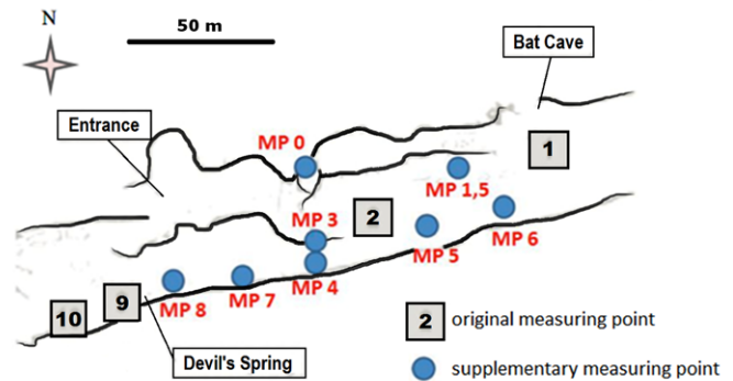
Figure 4. Location of the original measuring points MP1, 2, 9, and 10 and the later added points MP0, 1.5, and 2–8 in the front part of Carlsbad Cavern (based on Schwabe, 2013).
