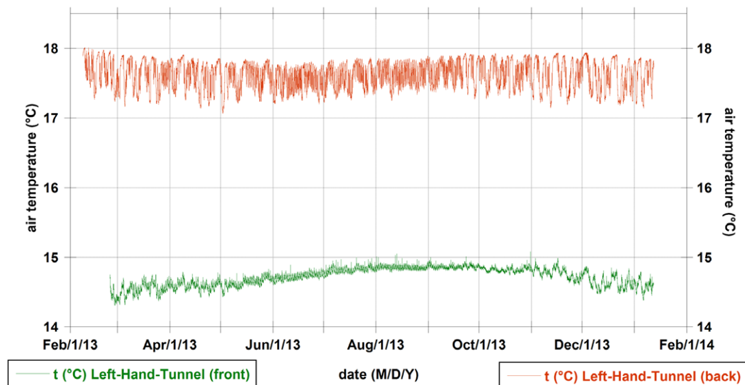
Figure 7. Records of the air temperature in the exterior (front, logger LHT-F) and the interior (back, logger LHT-B) parts of the Left Hand Tunnel inside Carlsbad Cavern from February 2013 to January 2014, recorded every 5 minutes.
