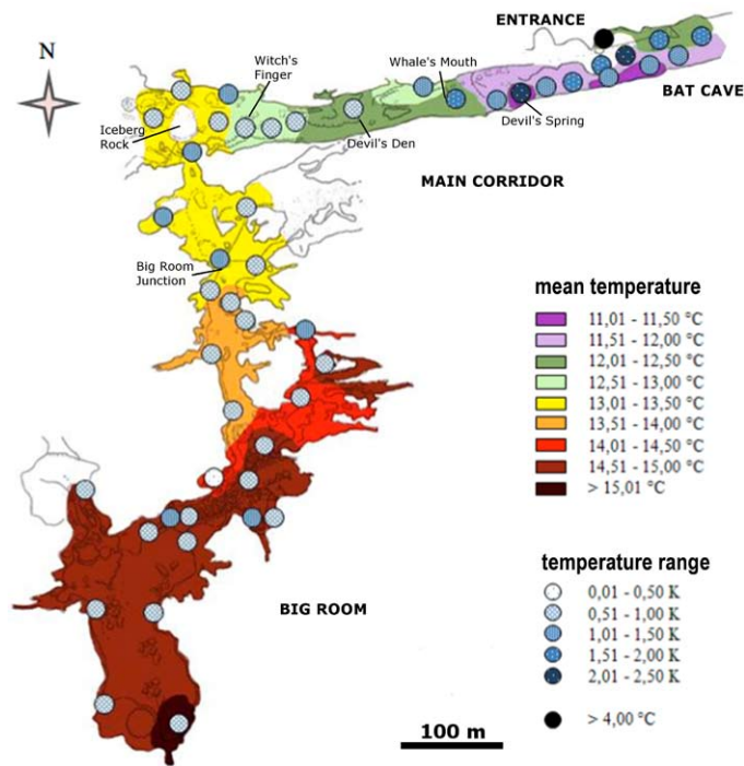
Figure 14. Depiction of the temperature conditions inside Carlsbad Cavern by temperature zones (colored areas) and the temperature ranges at Schwabe's measuring points (circle icons) in March-April 2011 (based on Schwabe, 2013).
