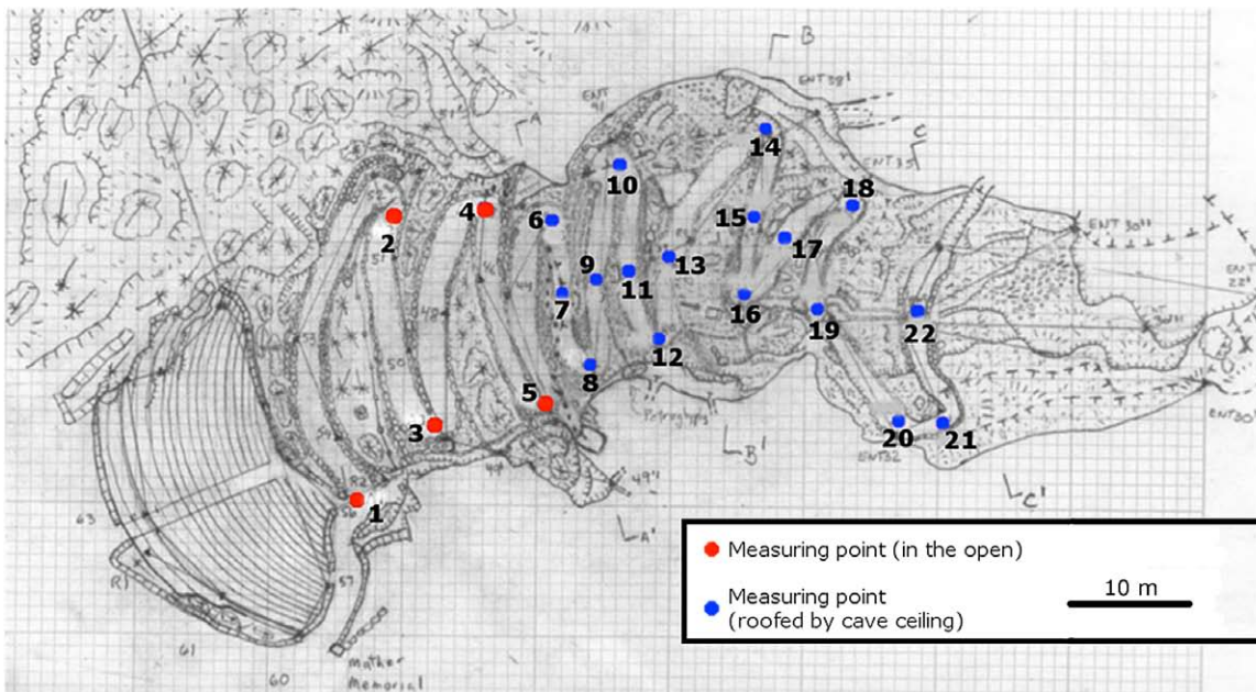
Figure 5. Positions of the outside measuring points A A 1–A A 22 in the area of the Natural Entrance of Carlsbad Cavern during Adam’s study (Adam, 2014).
