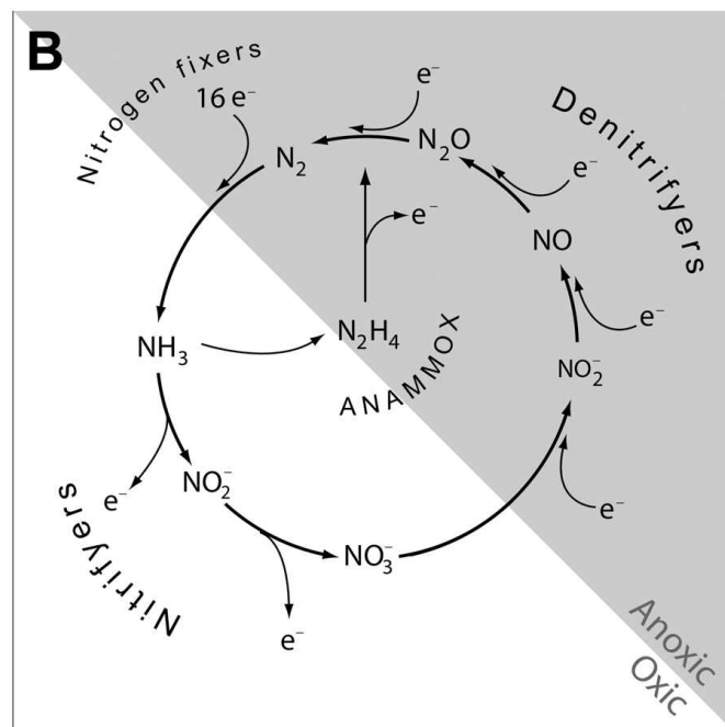
Figure 1. The degradation of urea and the nitrogen cycle. A. A simplification of the breakdown of urea by urease into ammonia. B. The nitrogen cycle not only provides nitrogen in a bioavailable form for plants and bacteria ( \text{NO}_3^- ), but the valency of the nitrogen species also allows them to serve as electron donors or electron acceptors in bacterial energy-generating processes. Ammonia is oxidized by nitrifying bacteria into nitrite and nitrate, while nitrate can be reduced by denitrifying bacteria to generate nitrous oxide and nitrogen gas. Under anaerobic conditions, ammonia can be directly oxidized to nitrogen gas by anaerobic ammonia-oxidizing (ANAMMOX) bacteria. In either case, either nitrogen gas from the nitrogen cycle or directly from the air can be made bioavailable by nitrogen-fixing bacteria in the form of ammonia.
